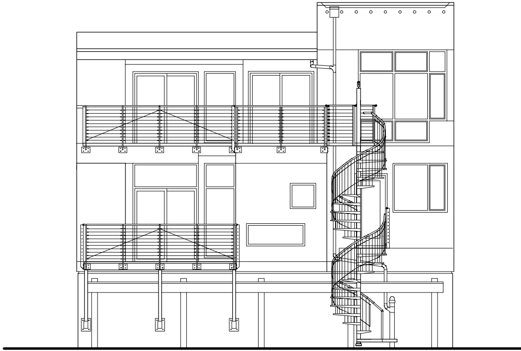
North Elevation
