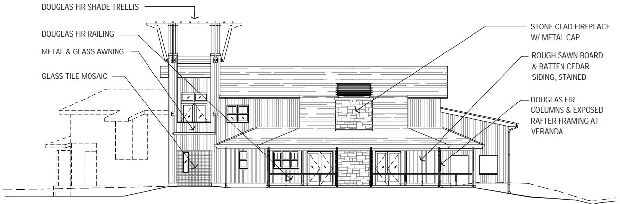
WEST ELEVATION
