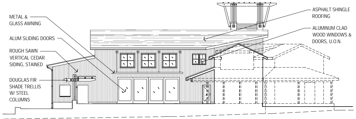
EAST ELEVATION
