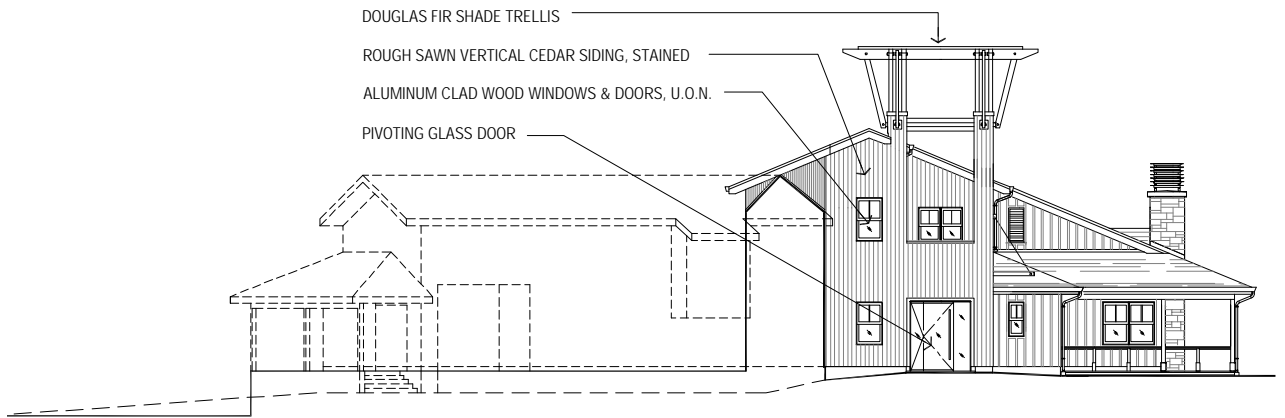
NORTH ELEVATION
