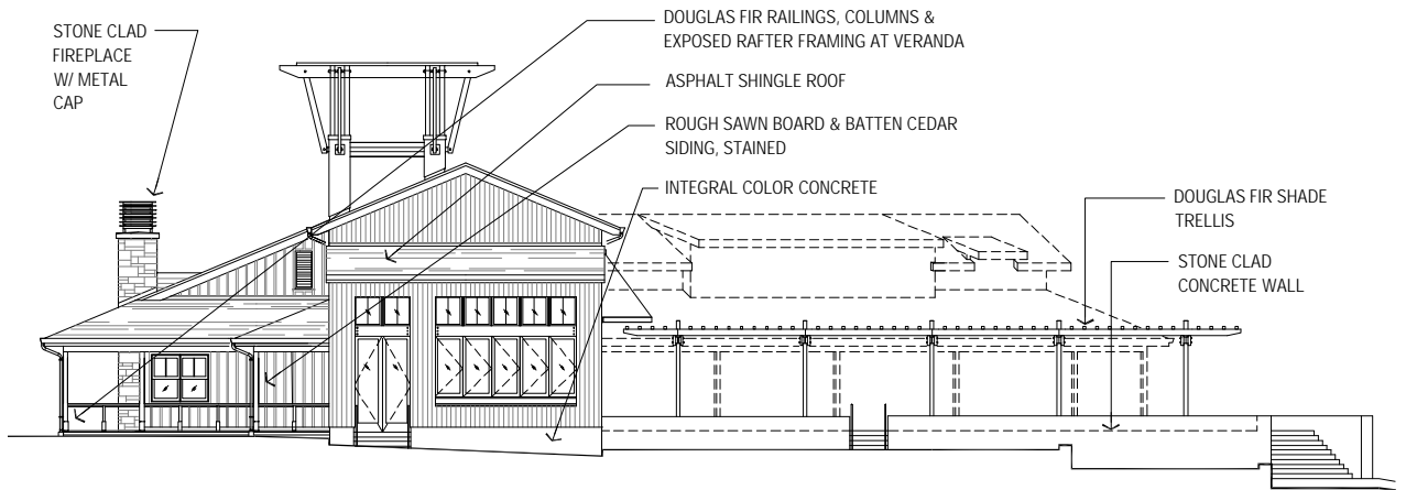
SOUTH ELEVATION
