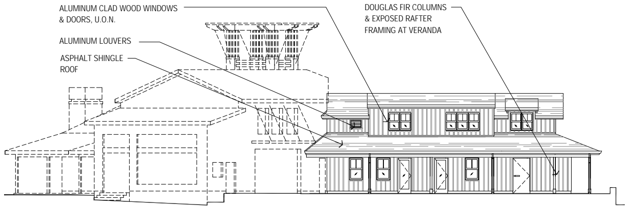
SOUTH ELEVATION - EAST WING
