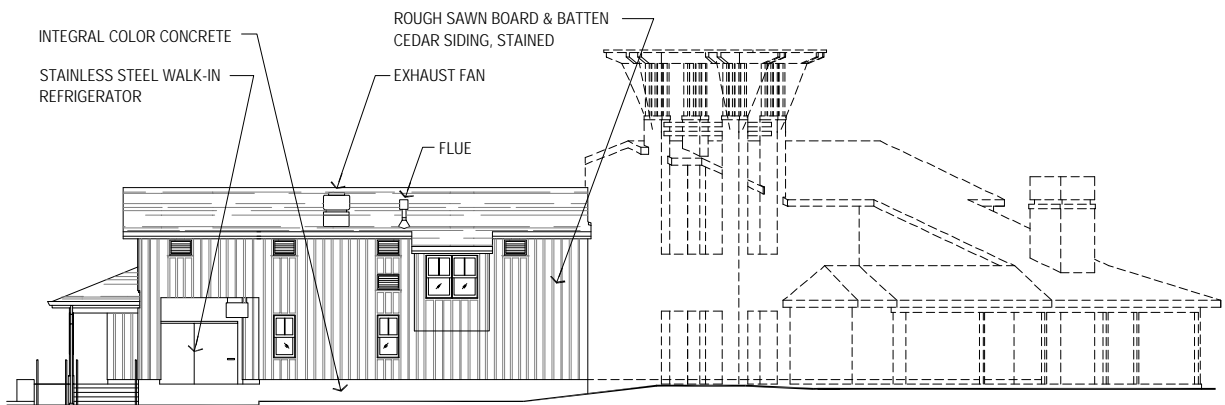
NORTH ELEVATION - EAST WING
