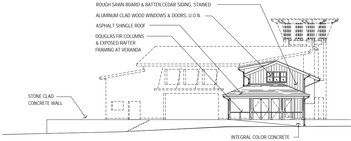
EAST ELEVATION - EAST WING
