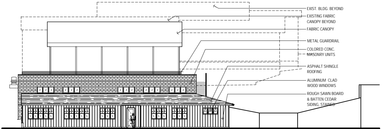
NORTH ELEVATION
