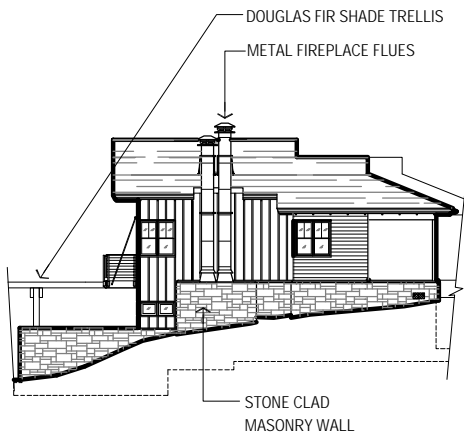
NORTH ELEVATION
