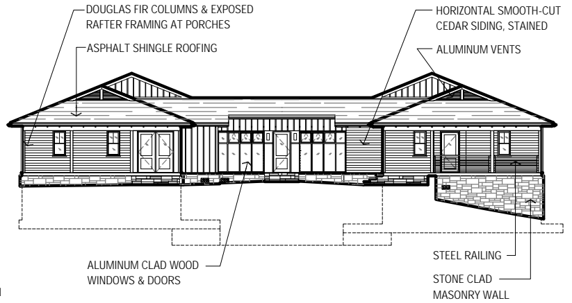
WEST ELEVATION
