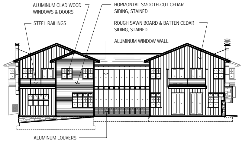
EAST ELEVATION
