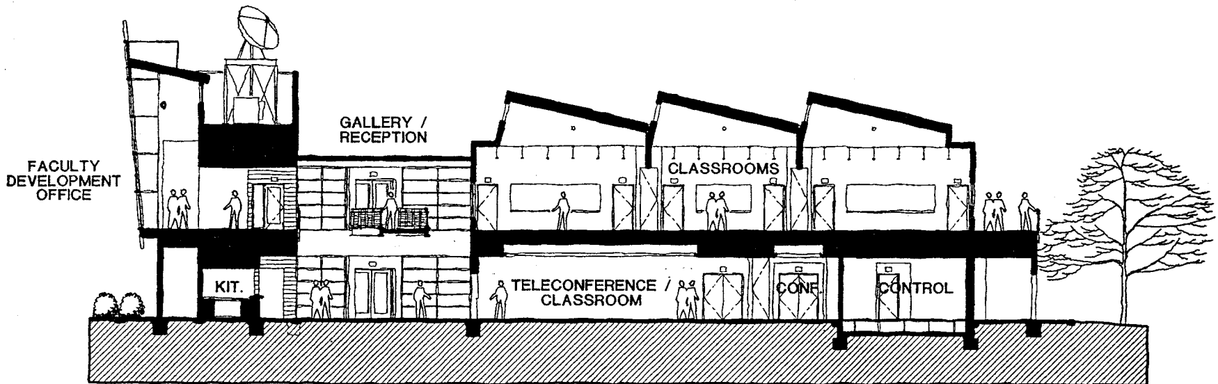
North - South Section 1/16" = 1'-0"
